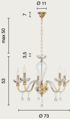
lampadario chandelier LP.ROXANNE/5 METEL: OLP0220
